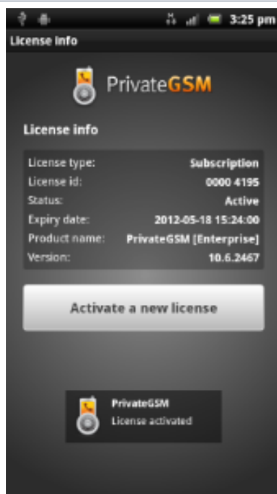
4. License registration
