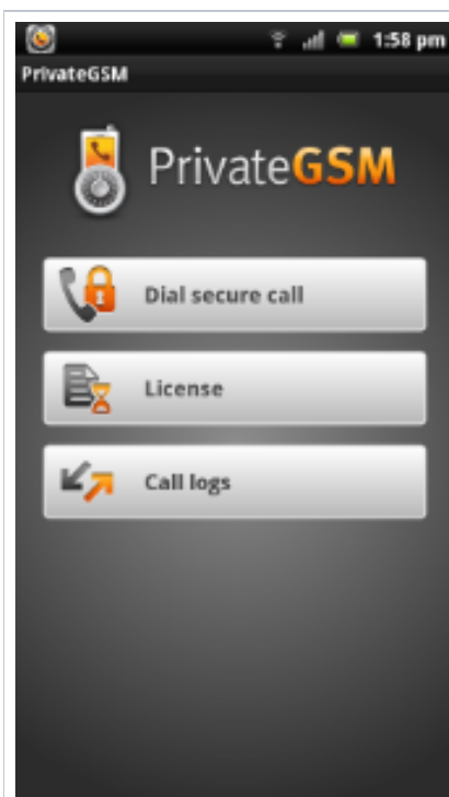
1. Select License
